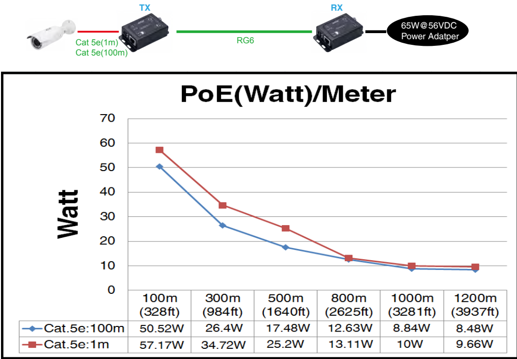
Power / Distance Chart
